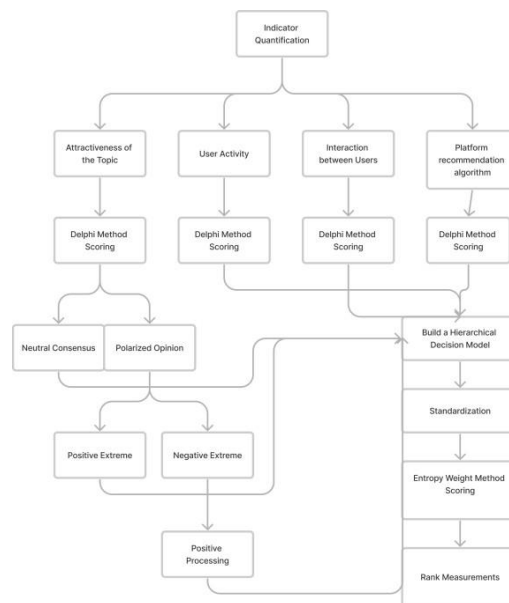
Figure 2.6: the main idea of modeling
